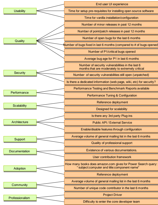
Figure 2: OpenBRR hierarchy of evaluation criteria.
