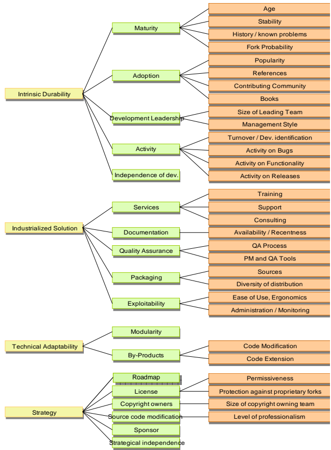
Figure 1: Generic criteria from QSOS version 1.6
